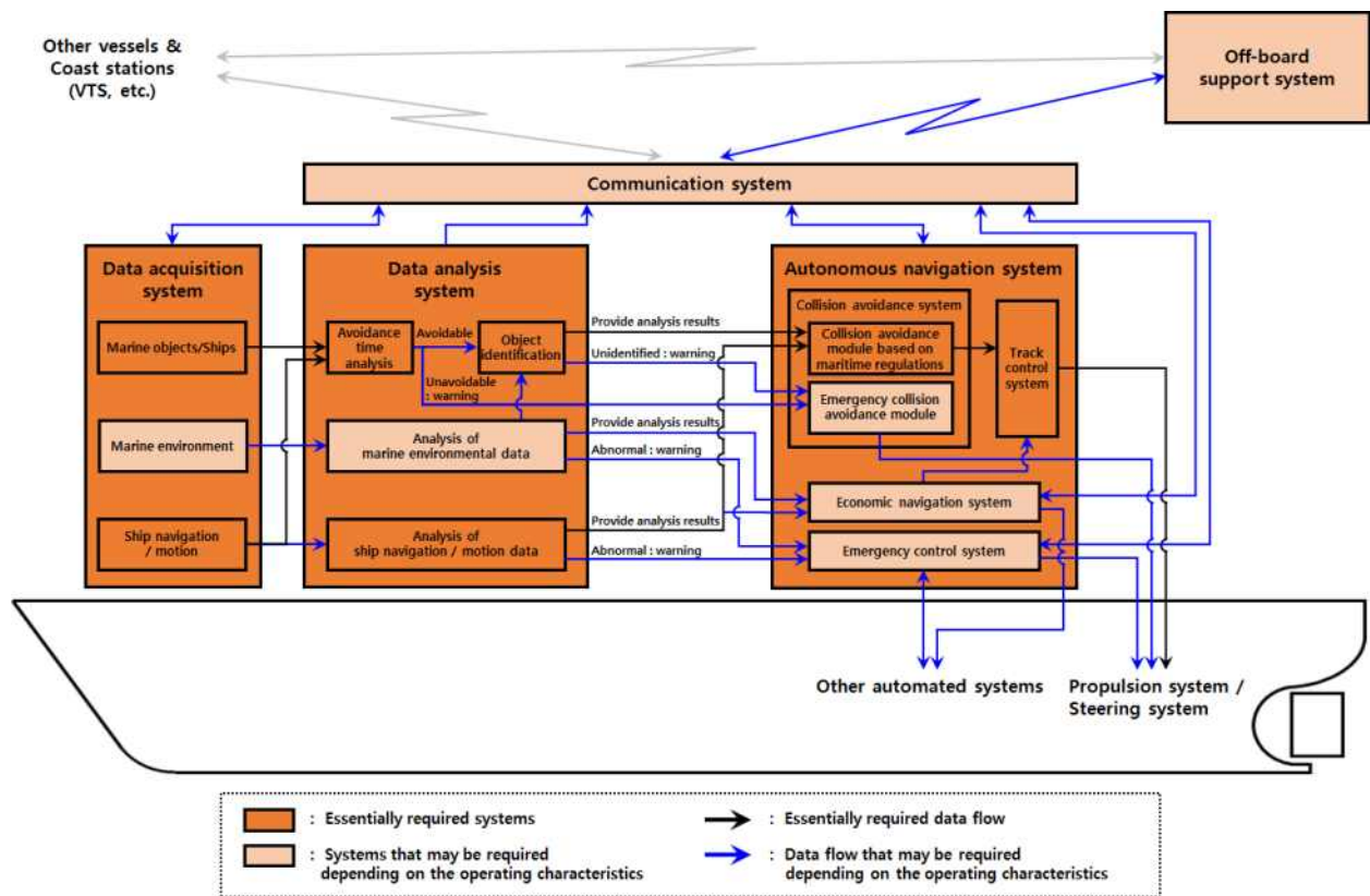
Fig 3.4 Autonomous system required for the ship of autonomy level 3 (AL 3)
